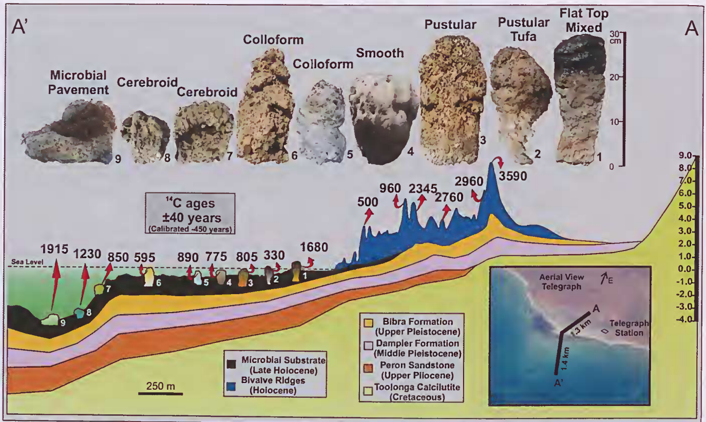
Figure 10 Regional cross-section based on DGPS (land) and multi-beam (water) surveys located north of Telegraph Station area with projected microbial samples and respective 14 C ages calibrated by subtracting 450 years from the conventional ages. The stratigraphy is based on boreholes drilled over the ridge system (in blue) and is projected offshore. The supratidal Hamelin Coquina storm ridge transect (morphology and ages) is shown for comparative purposes. Note basinward (upper surface) ages; also relict, emergent head 1 at landward end of transect. (Jahnert & Collins 2012 figure 10).
